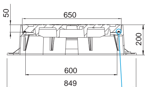
Joint EPDM
